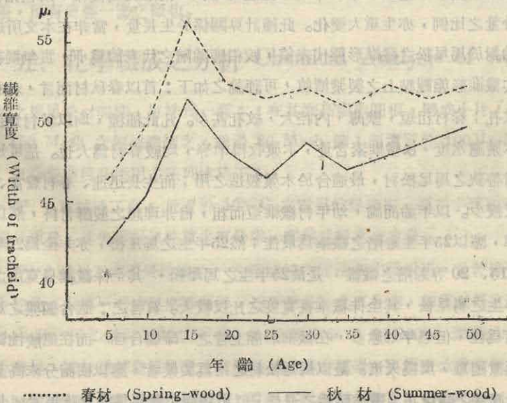
Fig. 3. The width of Chinese pine fiber in different ages
