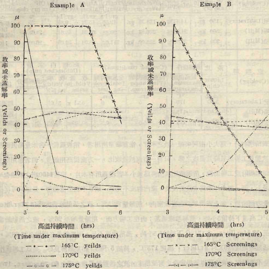
Eig 5. Curves shown the relations of yeilds and screenigns to cooking conditions in the pulping of Chinese pine
