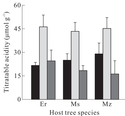
Fig. 2. Early evening (black bars), early morning (light-gray bars), and daytime decreases in (dark-gray bars) acidity (on a fresh mass basis) of leaves of the epiphytic orchid Bulbophyllum japonicum on 3 host tree species in a subtropical rainforest in northeastern Taiwan. The host species were Engelhardia roxburghiana (Er), Meliosma squamulata (Ms), and Machilus zuihensis (Mz). Data are presented as the mean and standard errors for 6 (Er), 5 (Ms), and 4 (Mz) trees per respective host species. For all three host species, leaf acidity in the morning was significantly greater than that in the evening ( p < 0.001 ), yet daytime decreases in acidity did not vary among the host species ( p > 0.05 ).
