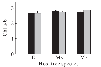
Fig. 4. Leaf chlorophyll (Chl) a/b ratios, in the morning (black bars) and at noon (light-gray bars), in leaves of the epiphytic orchid Bulbophyllum japonicum on 3 host tree species in a subtropical rainforest in northeastern Taiwan. The host species were Engelhardia roxburghiana (Er), Meliosma squamulata (Ms), and Machilus zuihensis (Mz). Data are presented as the mean and standard errors for 6 (Er), 5 (Ms), and 4 (Mz) trees per respective host species. None of the means at each time of measurement significantly differed ( p > 0.05 ).
