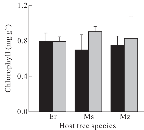
Fig. 3. Leaf chlorophyll concentrations (on a dry mass basis), in the morning (black bars) and at noon (light-gray bars), of leaves of the epiphytic orchid Bulbophyllum japonicum on 3 host tree species in a subtropical rainforest in northeastern Taiwan. The host species were Engelhardia roxburghiana (Er), Meliosma squamulata (Ms), and Machilus zuihensis (Mz). Data are presented as the mean and standard errors for 6 (Er), 5 (Ms), and 4 (Mz) trees per respective host species. None of the means at each time of measurement significantly differed ( p > 0.05 ).
