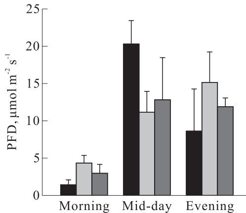
Fig. 1. Photosynthetic photon flux density (PPFD) at 3 times of day intercepted by the epiphytic orchid Bulbophyllum japonicum on 3 host tree species in a subtropical rainforest in northeastern Taiwan. The host species were Engelhardia roxburghiana (black bars), Meliosma squamulata (light-gray bars), and Machilus zuihensis (dark-gray bars). Data are presented as the mean and standard errors for six, five, and four trees per respective host species. None of the means at each time of measurement significantly differed (all p > 0.05 ).
