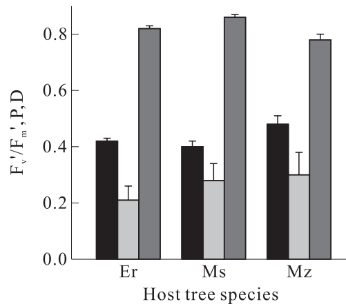
Fig. 6. Actual efficiency of energy conversion in photosystem II ( F_v'/F_m' ; black bars), energy dissipation in photosystem II via photochemistry (P; light-gray bars), and energy dissipation via nonphotochemical thermal means (D; dark-gray bars) at midday of leaves of the epiphytic orchid Bulbophyllum japonicum on 3 host tree species in a subtropical rainforest in northeastern Taiwan. The host species were Engelhardia roxburghiana (Er), Meliosma squamulata (Ms), and Machilus zuihensis (Mz). Data are presented as the mean and standard errors for 6 (Er), 5 (Ms), and 4 (Mz) trees per respective host species. None of the means at each time of measurement significantly differed ( p > 0.05 ).
