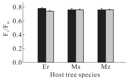
Fig. 5. Intrinsic efficiency of energy conversion in photosystem II ( F_v/F_m ) early in the morning (black bars) and at noon (light-gray bars) of leaves of the epiphytic orchid Bulbophyllum japonicum on 3 host tree species in a subtropical rainforest in northeastern Taiwan. The host species were Engelhardia roxburghiana (Er), Meliosma squamulata (Ms), and Machilus zuihensis (Mz). Data are presented as the mean and standard errors for 6 (Er), 5 (Ms), and 4 (Mz) trees per respective host species. None of the means at each time of measurement significantly differed ( p > 0.05 ).
