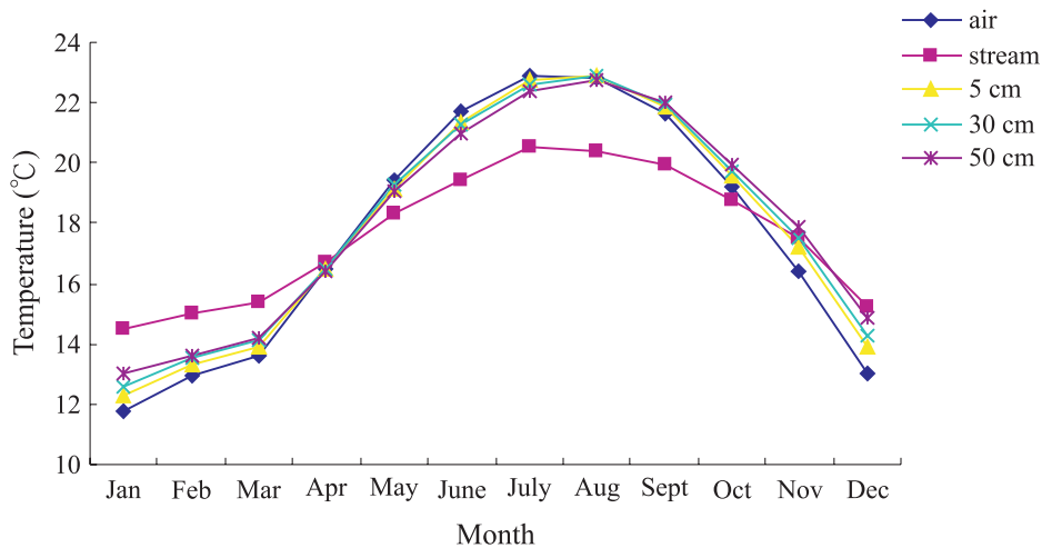
Fig. 3. Yearly temperature fluctuations in a riparian area of Harpen Creek.
