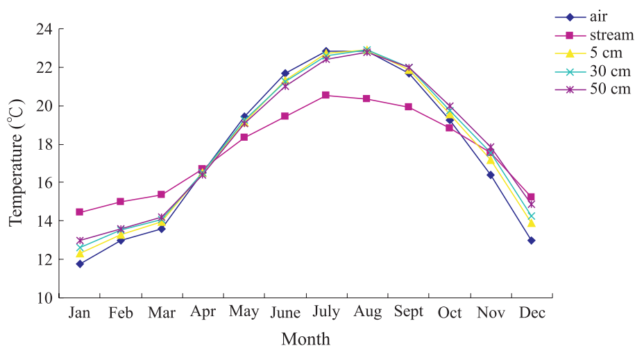
Fig. 2. Monthly average temperatures for air, streamflow, and soils at different depths for a riparian area of Harpen Creek.
