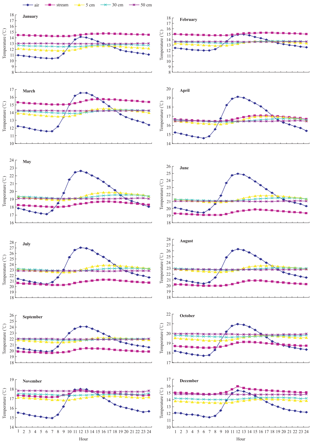
Fig. 4. Hourly temperatures of each month for a riparian area of Harpen Creek.
